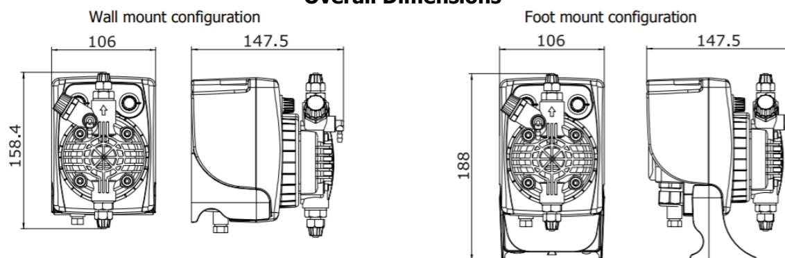
Overall Dimensions
