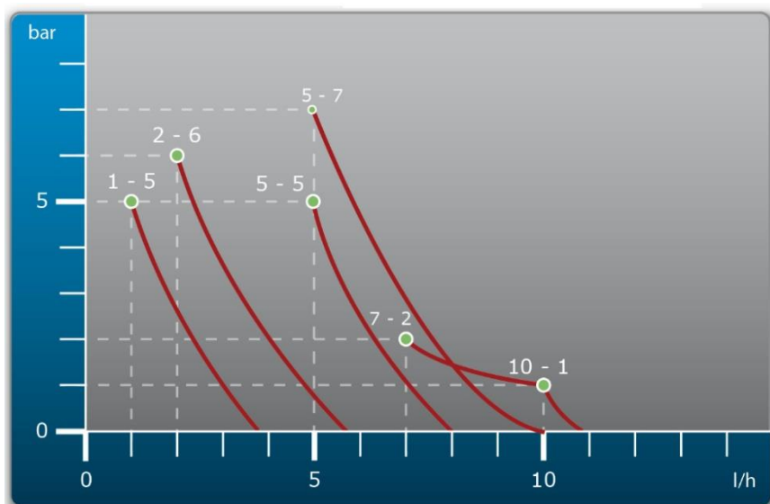
Pressure (bar) – Flow Rate (l/h) Chart
