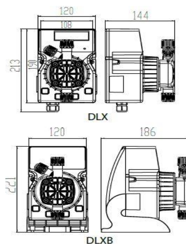
Overall Dimensions
